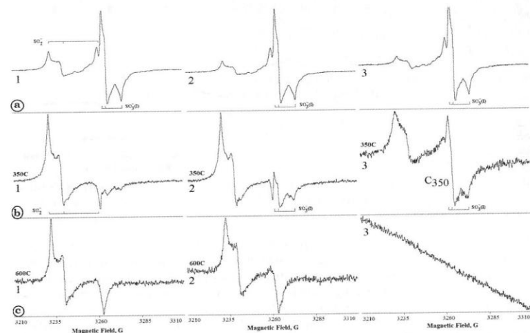
Fig.3. EPR spectra of radical ions \text{SO}_2^{\cdot-} and \text{SO}_3^{\cdot-} (I): a) at room temperature; b) after 350^\circ\text{C} annealing; c) after 600^\circ\text{C} annealing. Location selection is indicated by the numbers 1, 2, 3.
