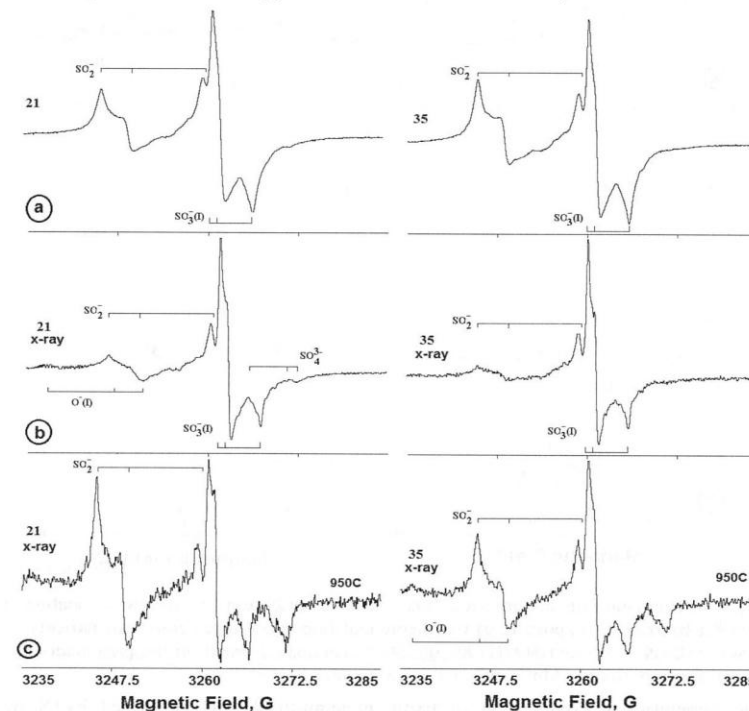
Fig.4. EPR spectra of radical ions barite mineralization of the sample 21 and 35: a) the original rock; b) after irradiation source rocks; c) after irradiation at 950^\circ\text{C} heated rocks.
