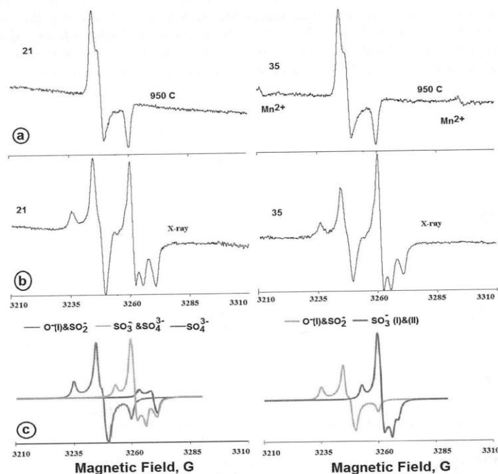
Fig.5. EPR radical ions in barite rock (sample number 21 and 35): a) after annealing at 950 °C; b) after re- exposure; c) the theoretical line spectral envelope ion radicals O^{\cdot-} & SO_2^{\cdot-} , SO_3^{\cdot-} & SO_4^{\cdot-} and SO_3^{\cdot-}(I) & (II) , SO_4^{\cdot-} , calculated based on the parameters [2]. Line trace impurity ion Mn^{2+} are listed in carbonates host rock.
