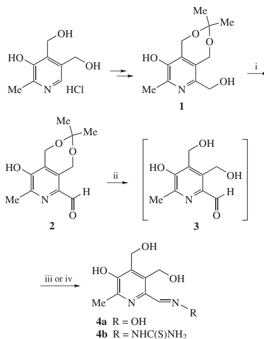
Scheme 1 Reagents and conditions: i, MnO 2 , EtOH, H 2 O, 40°C, 6 h; ii, HCl, H 2 O, EtOH, 20°C, 8 h; iii, NH 2 OH·HCl, AcONa, H 2 O, reflux, 5 min; iv, NH 2 NHC(S)NH 2 , EtOH, reflux, 10 h.
