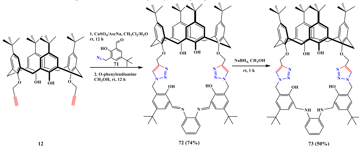
Fig. 21. Synthetic route for macrocycle 73 , responsive to \text{H}_2\text{PO}_4^-
