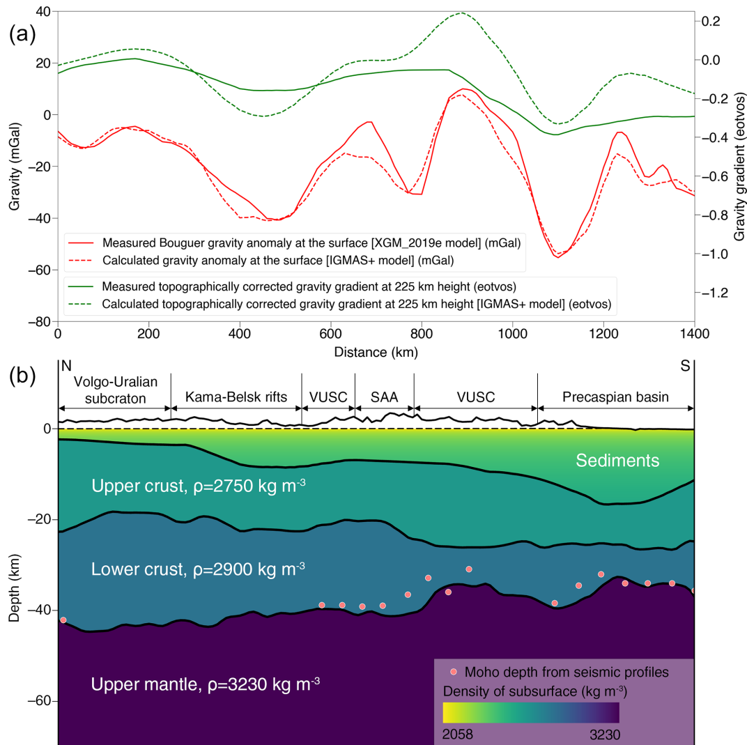
Figure 13. Measured and calculated Bouguer gravity anomalies and the topographically corrected vertical gravity gradient anomalies from the crustal model (a) and IGMAS+ model north–south cross-section in the eastern part of Volgo–Uralia (b) – see Fig. 3 for the reference on the map. Subsurface is vertically exaggerated by the factor of 10 and topography is by the factor of 100. VUSC stands for Volgo–Uralian subcraton and SAA for Sernovodsk–Abdulinsk Aulacogens.
