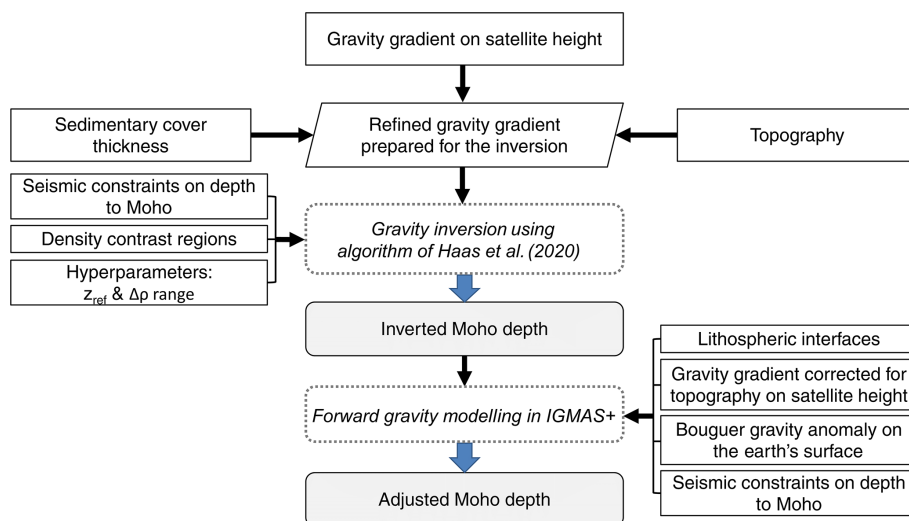
Figure 2. Schematic workflow of the study. The initial step is to prepare the gravity data for the inversion by subtracting the sedimentary cover effect from the topographically corrected vertical gravity gradient. Then it can be followed by a subsequent gravity inversion with laterally variable crust–mantle density contrast (Haas et al., 2020). The inverted Moho depth is incorporated along with other lithospheric interfaces as well as seismic and gravity constraints in IGMAS+ software (Schmidt et al., 2020; Götze and Lahmeyer, 1988). The interfaces are modified to fit the existing gravity and seismic constraints providing the adjusted Moho depth of the region.
