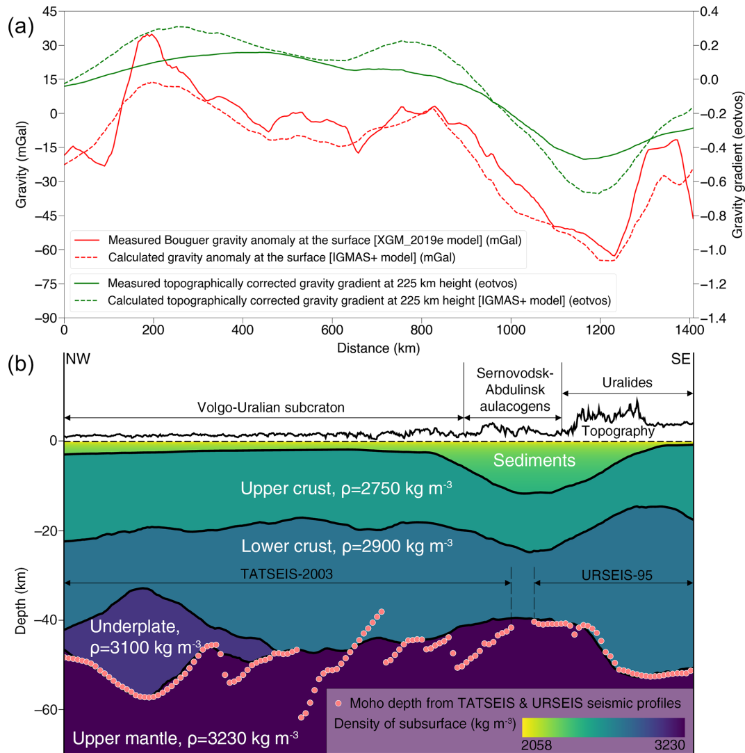
Figure 12. Measured and calculated Bouguer gravity anomalies and the topographically corrected vertical gravity gradient anomalies from the crustal model (a) and IGMAS+ model cross-section along TATSEIS-2003 and URSEIS-95 deep reflection profiles (b) – see Fig. 3 for the reference on the map. Subsurface is vertically exaggerated by the factor of 10 and topography is by the factor of 100.
