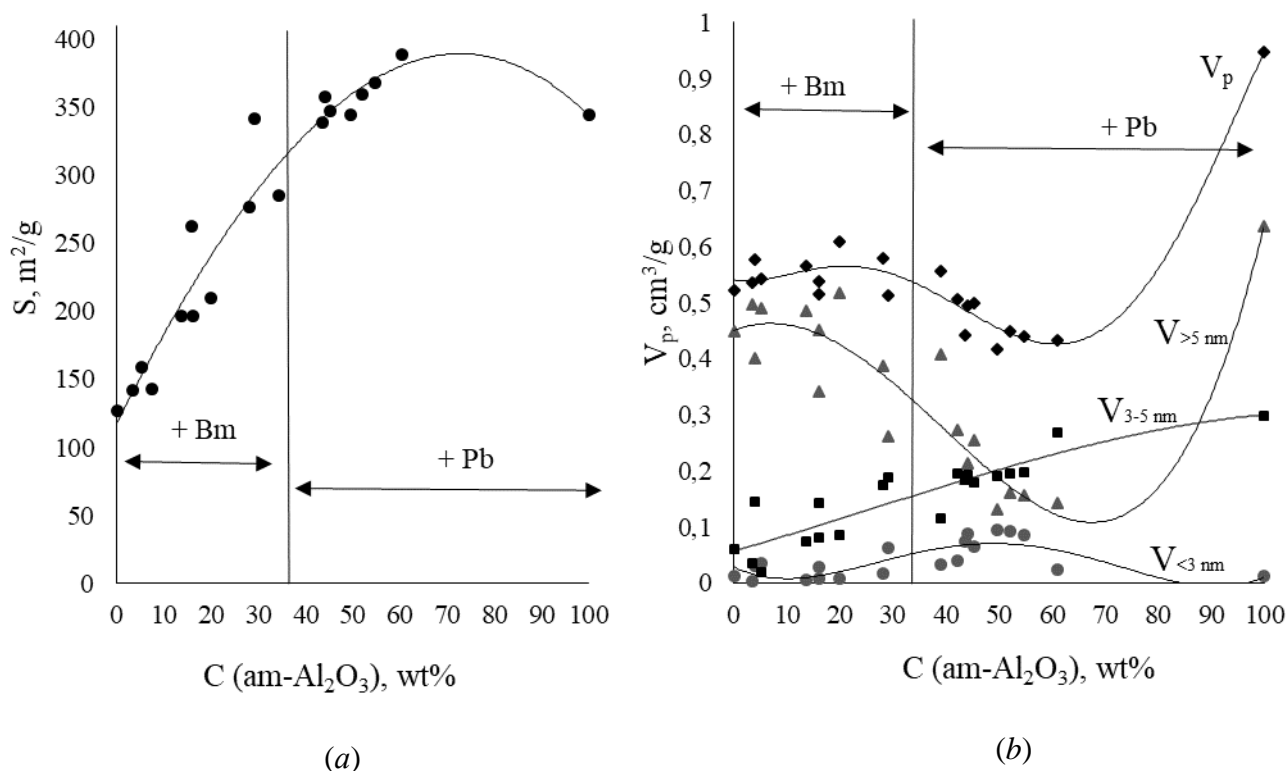
Figure S4 (a) Specific surface area S and (b) pore volume V_p of aluminum monohydroxides formed under hydrothermal condition from amorphous alumina.
