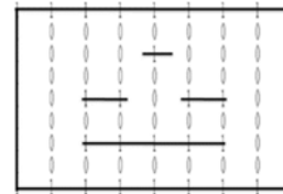
Fig. 7 images conversion.
