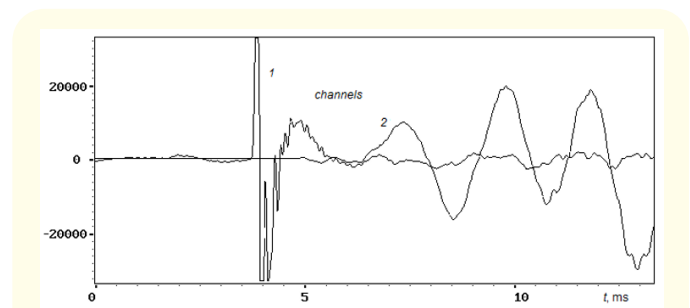
Figure 2: An example of the temporal realization for the granite sample in the ULF frequency range with using the seismic sensor. Drop height of a steel ball weighing 80g to sample is 50 cm.
