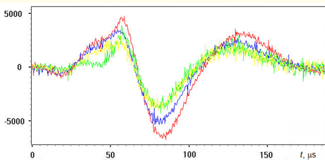
Figure 10: Electrical signal at the four impacts on the mudstone sample.
