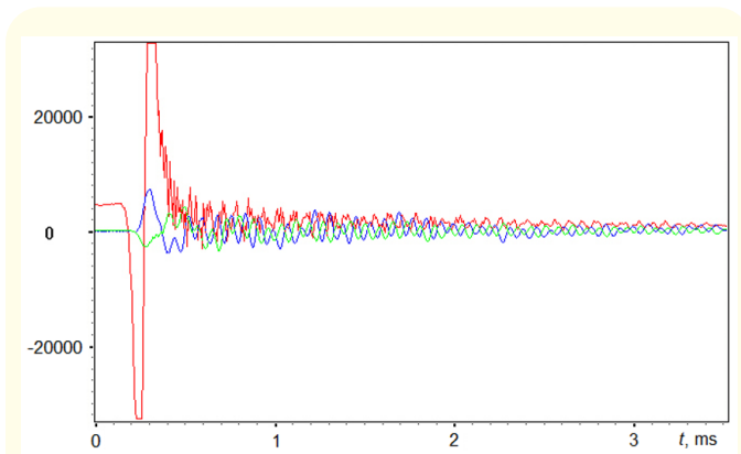
Figure 6: Oscillograms of the electrical (red line) and two seismic (blue and green lines) components.
