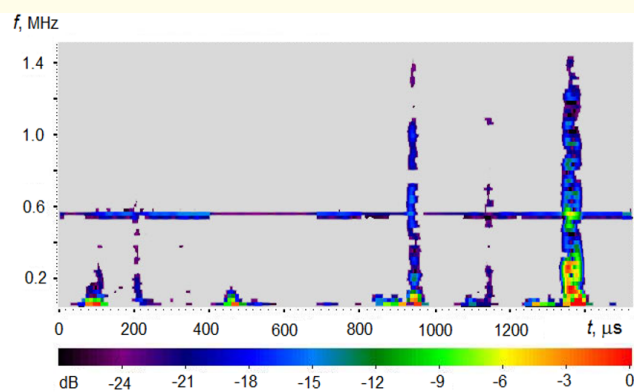
Figure 14: Spectrograms of the impacts shown in figure 13. The correspondence of the spectra to the realizations shown in figure 13: 0 - 300 \mu\text{s} - red, 400 - 700 \mu\text{s} - blue, 800 - 1000 \mu\text{s} - green, 1000 - 1200 \mu\text{s} - yellow, and 1200-1500 \mu\text{s} - pink, respectively.
