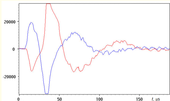
Figure 12: Oscillograms of two impacts on quartz sample at different angles: red line corresponds to the inclination of the sample plane at an angle of about 20 degrees to the horizontal one, blue line - the impact is strictly perpendicular.
