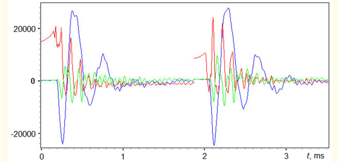
Figure 8: Oscillograms of two impacts on a granite sample: red line - the electrical signal, blue and green lines - two seismic components.
