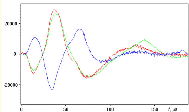
Figure 11: Electrical signal at the three impacts on the sample of mudstone with a quartz core.
