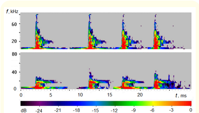
Figure 9: Spectrograms of the impacts on a granite sample corresponding to the oscillograms shown in figure 8.
