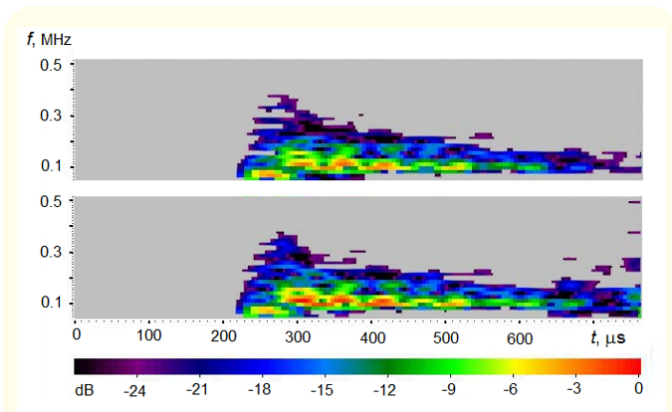
Figure 5: Spectrograms of two responses from a quartz sample.
