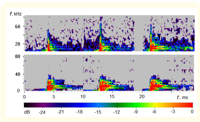
Figure 7: Spectrograms of three impacts on a quartz sample.
