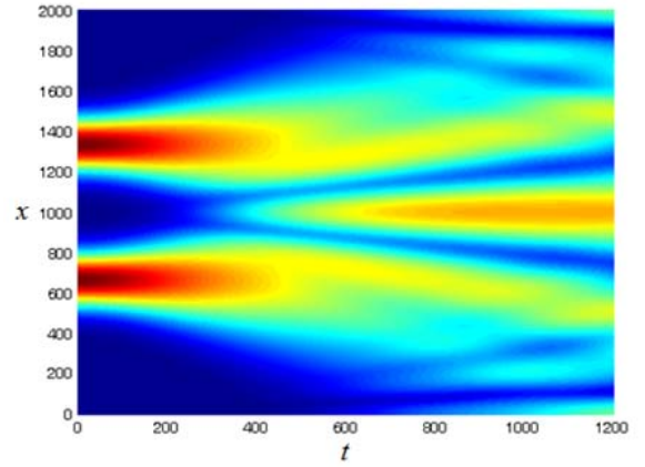
Fig. 2. Evolution of a Gaussian soliton-like envelop pulse (b) for A=1, l=4; \beta=0.5, \gamma=0 .
