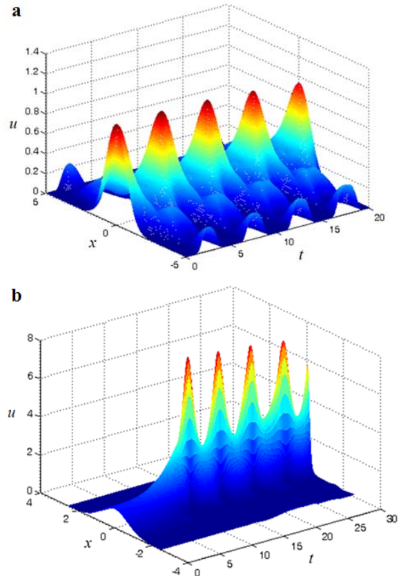
Fig. 3. Evolution of a Gaussian soliton-like envelop pulse in nonstationary medium at \alpha, f'=0 : a) \beta = 0.5, \gamma = -1+0.01\sin 2\pi t ; b) \gamma = -1, \beta(t) = -0.5 for t \leq 5 and \beta(t) = 0.5(1+0.2\sin 2\pi t) for t > 5 ; the cases of negative nonlinearity.
