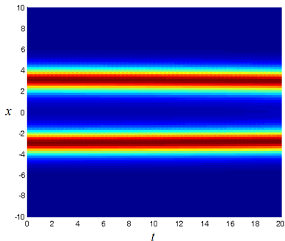
Fig. 5. Absence of interaction of the GNLS pulses (stationary medium) at \gamma = -1 , \beta = 0.05 ; the case of negative nonlinearity.
