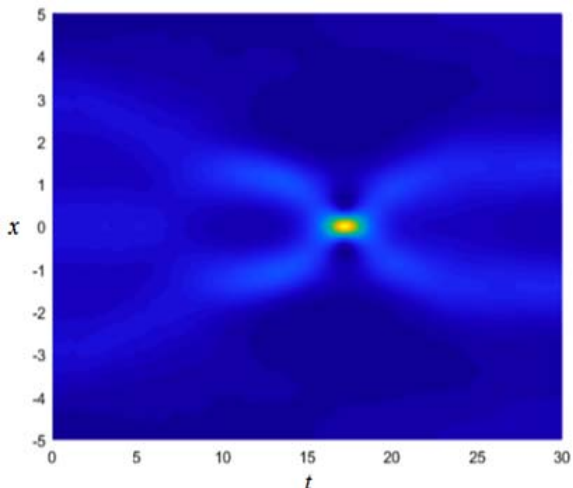
Fig. 4. Interaction of three GNLS pulses (stationary medium) at \gamma = -1 , \beta = 0.25 ; the case of weak negative nonlinearity.
