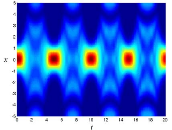
Fig. 5. Evolution of a 1D Gaussian envelop pulse in nonstationary medium at \beta = 0.5 , \gamma = -1+0.01\sin 2\pi t .
