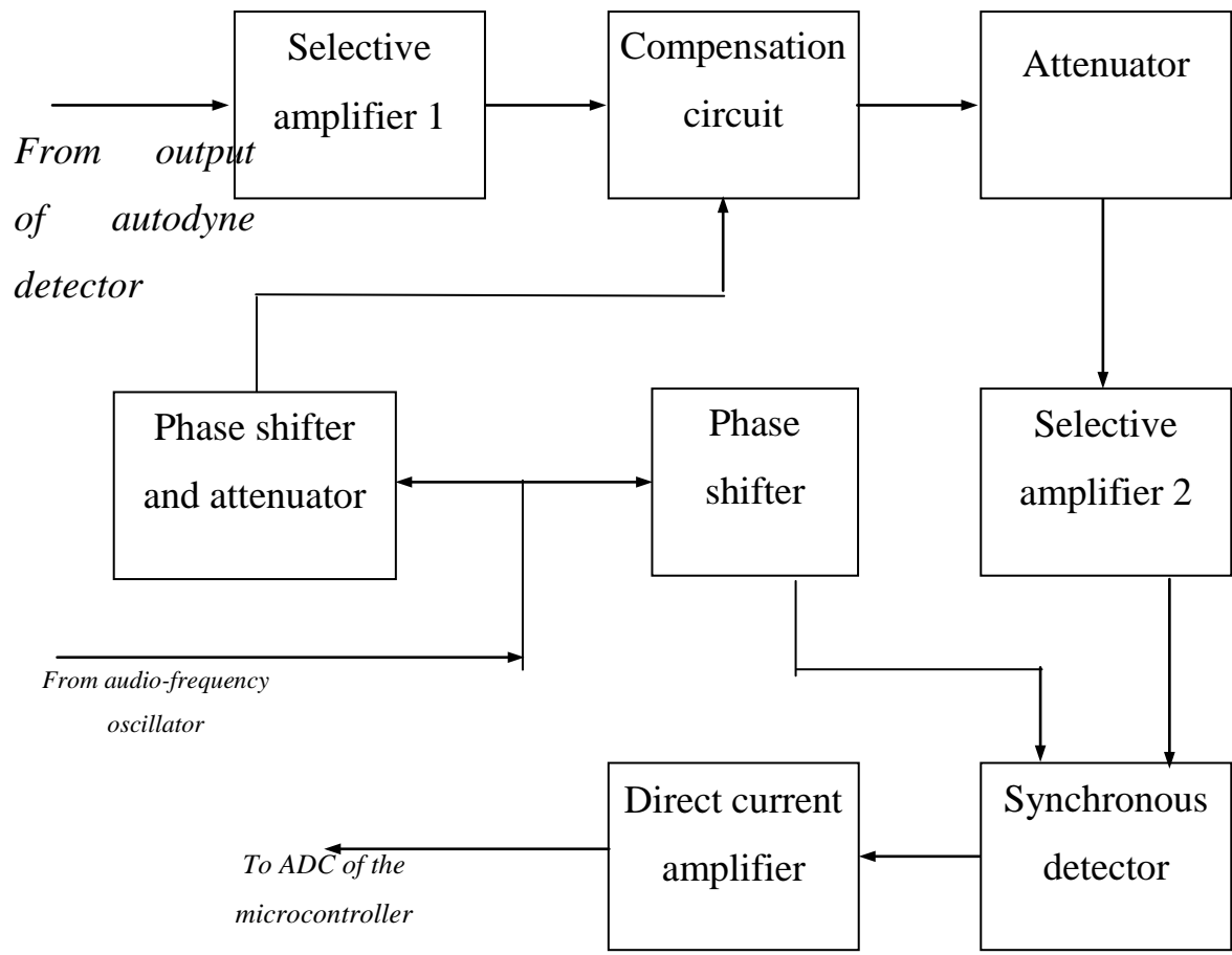
Fig. 11. Block diagram of the recording device
