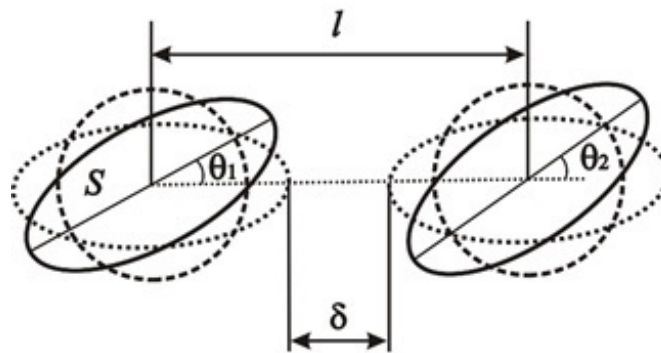
Figure 2. Illustration to definition of the initial state parameters of vortex system
