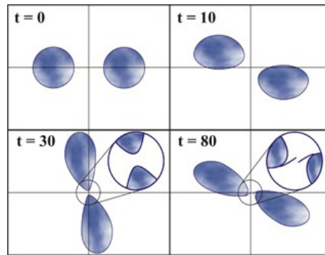
Figure 1. Formation of filaments of vorticity
