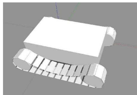
Fig. 3. Generic robot's main body tracks prototype modeling with Gazebo-tracks package
