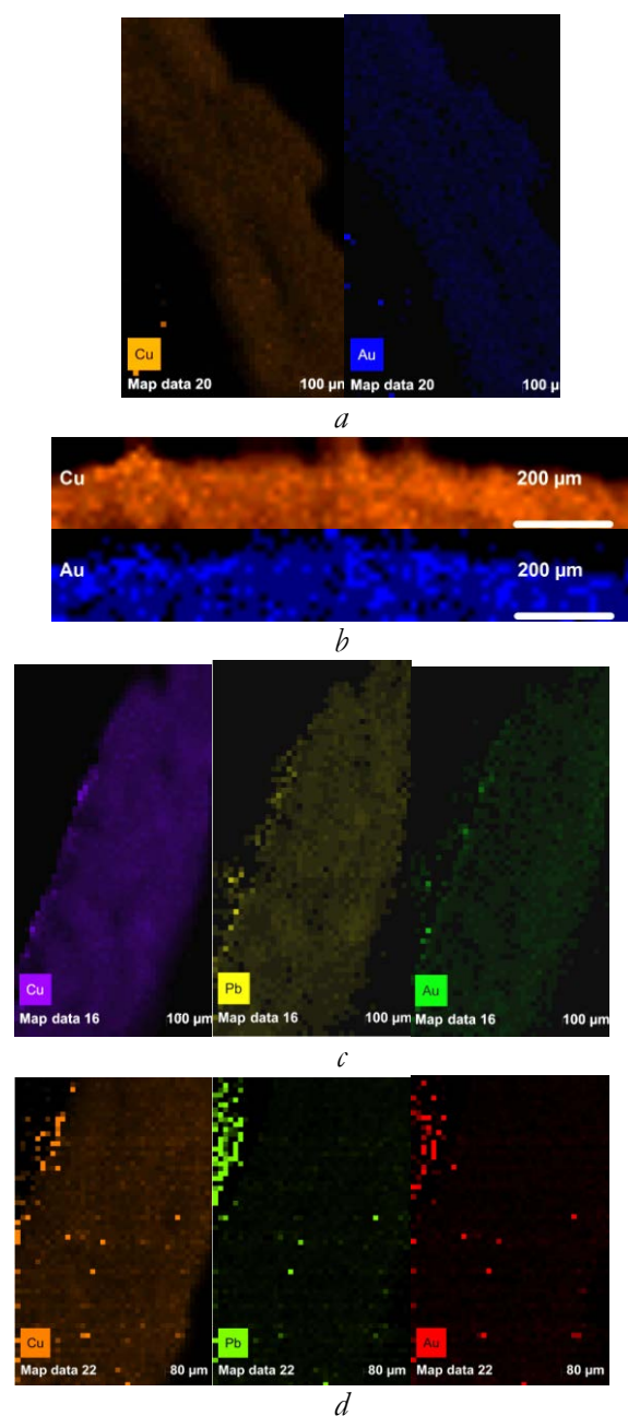
Figure 5. Elemental distribution across coin fractures: a – coin No.1 Cu and Au; b – coin No.3 Cu and Au; c – coin No.5 Cu, Au and Pb; d – coin No.6 Cu, Au and Pb.
