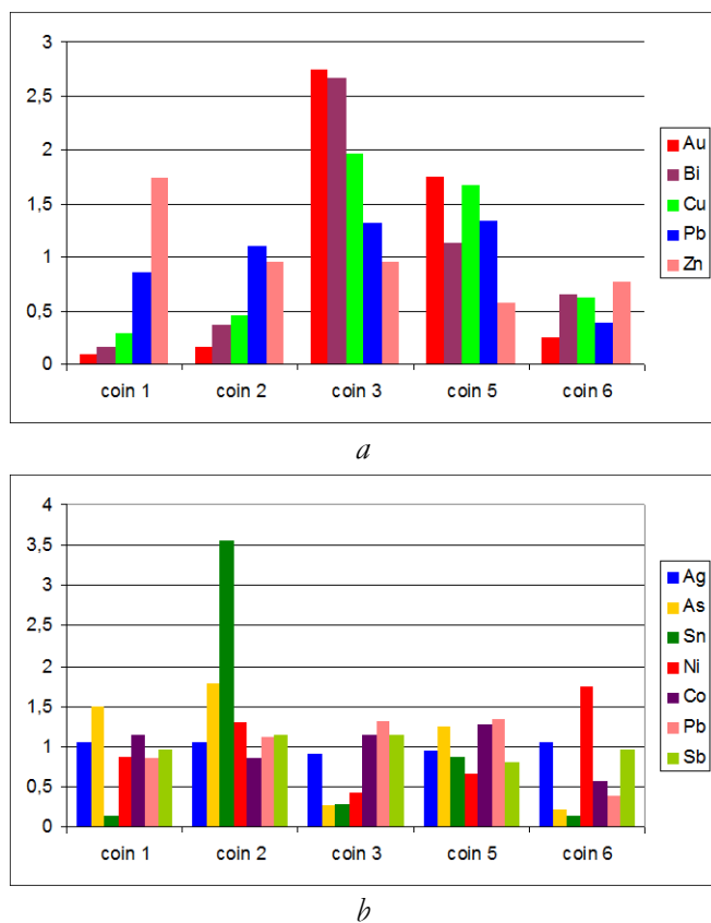
Figure 4. Diagrams of relative concentrations: a – Au, Bi, Cu, Pb, Zn; b – Ag, As, Sn, Ni, Co, Pb, Sb.
